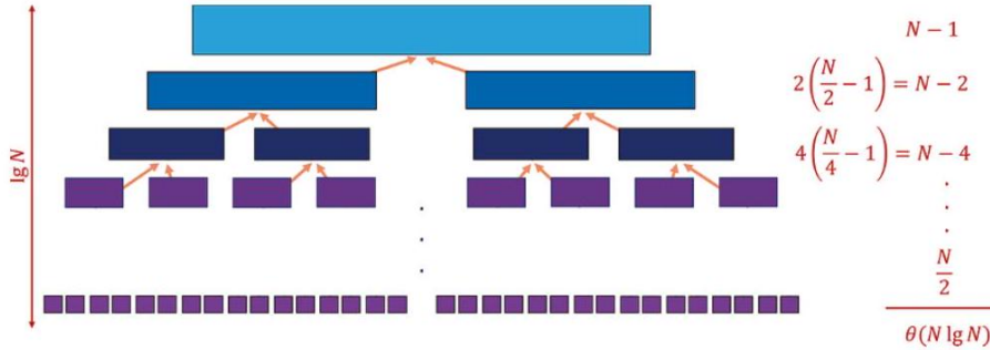
Figure 8.3: The recursion tree for mergesort. The tree has height \lceil \log_2 n \rceil , and the cost of the merging operations on each level are \Theta(n) , yielding an \Theta(n \log n) time algorithm.
